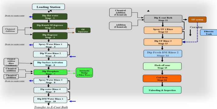
Process Flow Of CED Line ( 14 Tank Process )
